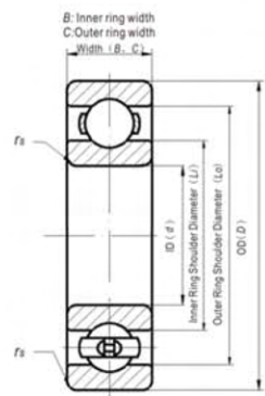
Dimensions list of deep groove ball bearing
